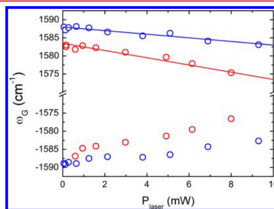
Figure 7. Power dependence of the G band frequencies \omega_G for tBLG (blue) and AB-BLG (red). Positive and negative values stand for Stokes and anti-Stokes peaks, respectively. The lines are fit to the Stokes data, given by \omega_G^{\text{tBLG}} = 1588.0 - 0.5P_{\text{laser}} (blue) and \omega_G^{\text{AB-BLG}} = 1583.5 - 1.0 P_{\text{laser}} (red).
