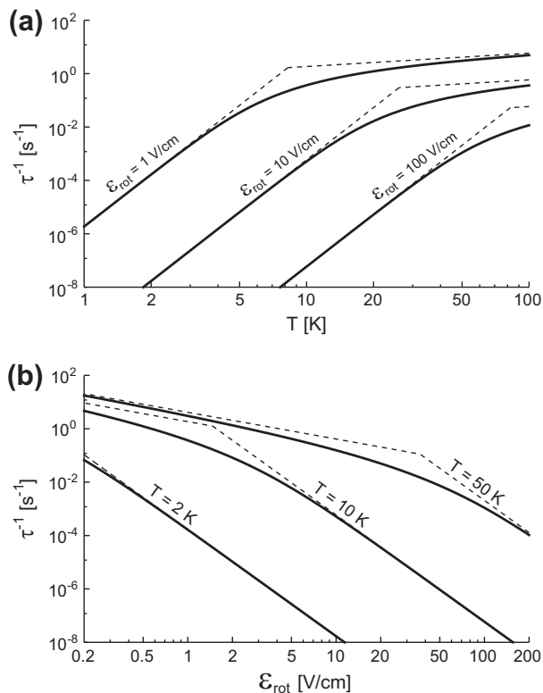
Fig. 12. Inverse coherence times, \tau^{-1} , due to geometric phases accumulated during ion-ion collisions as a function of (a) collision energy in temperature units and (b) \epsilon_{\text{rot}} . Dotted lines are approximations given in Eqs. (87) and (89). Solid lines are more involved estimates based on integrals over collision parameters, but are still based on approximations so as to be conservative. The ion density was taken to be n = 1000 \text{ cm}^{-3} .
