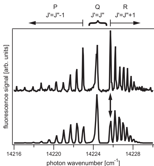
Fig. 4. Laser induced fluorescence (LIF) spectroscopy. The top trace is experimental data for a newly detected neutral \text{HfF} transition: [14.2] \mid \Omega = 3/2 \mid v' = v'', J' \rangle \leftarrow X^2\Delta_{3/2} \mid v'', J'' \rangle . The transition highlighted with a vertical arrow originates from the rotational ground state. The bottom trace is a theoretical prediction assuming a rotational temperature of 5 K. The traces are offset vertically for clarity.
