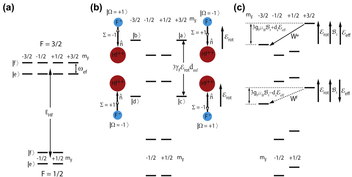
Fig. 1. Energy levels of \text{HfF}^+ in the ^3\Delta_1, J = 1 state including hyperfine structure associated with the fluorine I = 1/2 nucleus. A and \Sigma are defined as the projection along the molecular axis of the electronic orbital angular momentum, and spin, respectively. \Omega = A + \Sigma . (a) In zero electric field, the eigenstates of the system are states of good parity, |e\rangle = (|\Omega = +1\rangle - |\Omega = -1\rangle)/\sqrt{2} and |f\rangle = (|\Omega = +1\rangle + |\Omega = -1\rangle)/\sqrt{2} , separated by a small A -doublet splitting. (b) An electric field, \mathcal{E}_{rot} , mixes the parity eigenstates yielding states with well defined \Omega . (c) A small magnetic field lifts the degeneracy between states with the same value of m_F\Omega . A permanent electron electric dipole moment further breaks this degeneracy, but with opposite sign for the upper (solid arrow) and lower (dotted arrow) transition. Energy splittings not to scale.
